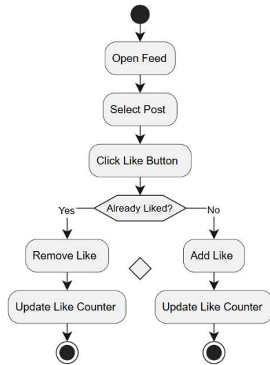
Figure 34- Activity Diagram – Like Post
