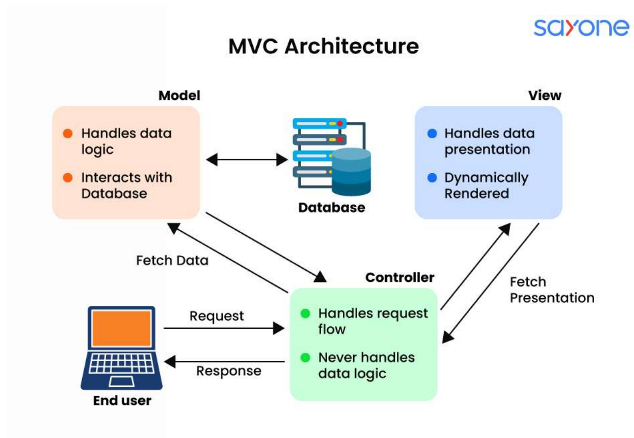
Figure 3- MVC Architecture of the UniSphere System
