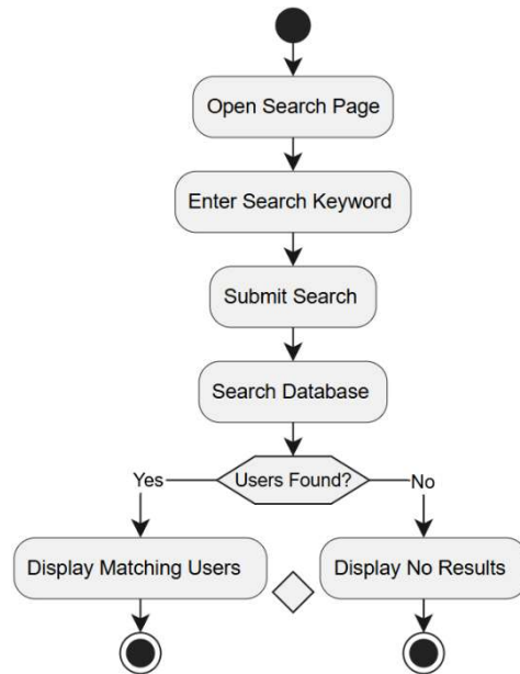
Figure 38- Activity Diagram – Search Users
