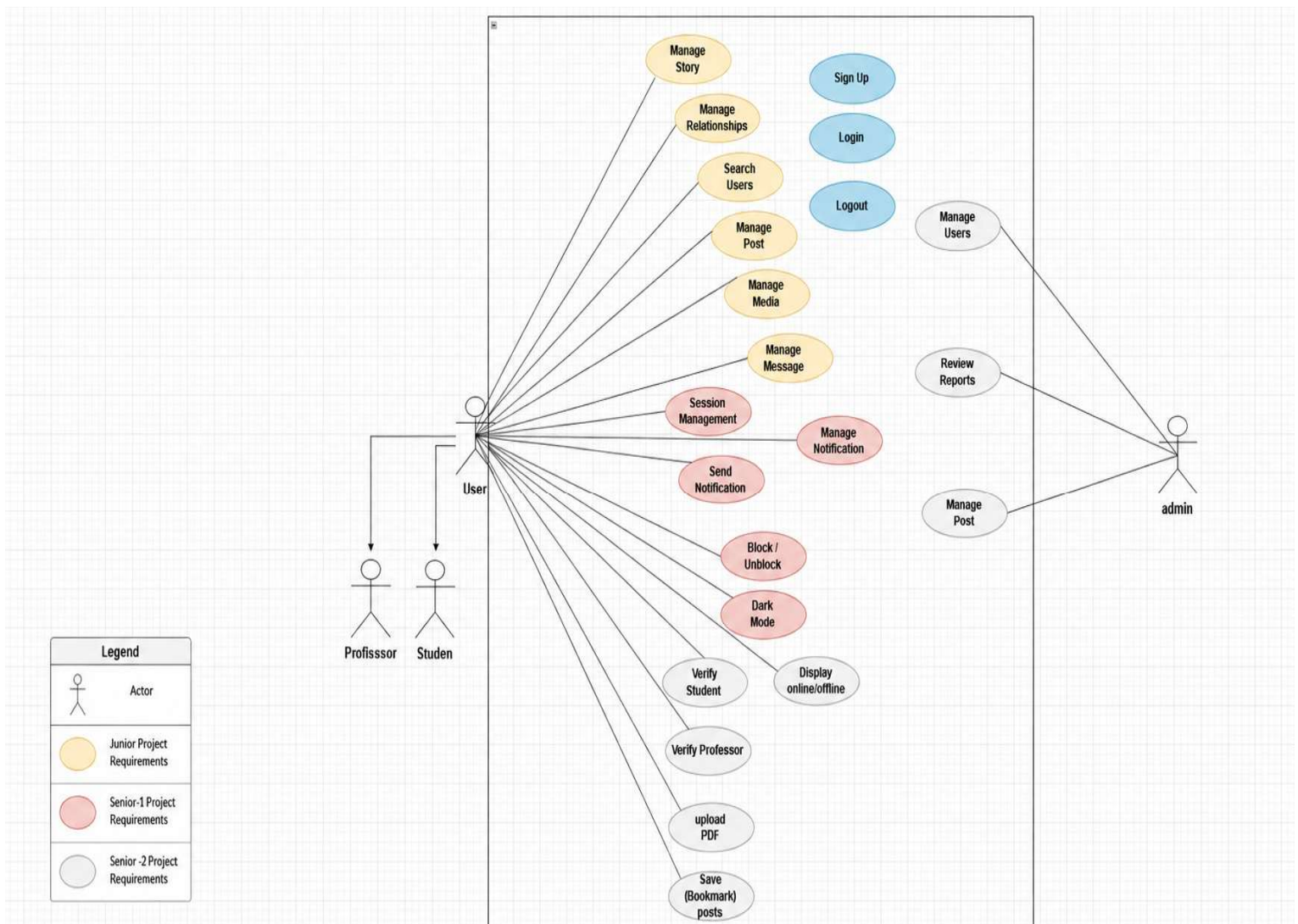
Figure 6- Use Case Diagram of the UniSphere System
