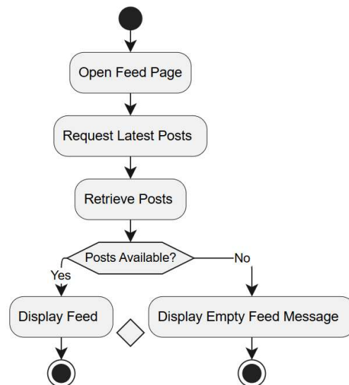
Figure 39- Activity Diagram – View Feed
