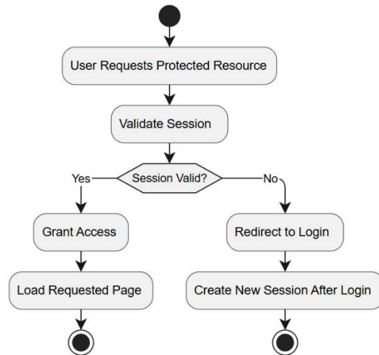
Figure 46- Activity Diagram – Manage User Sessions
