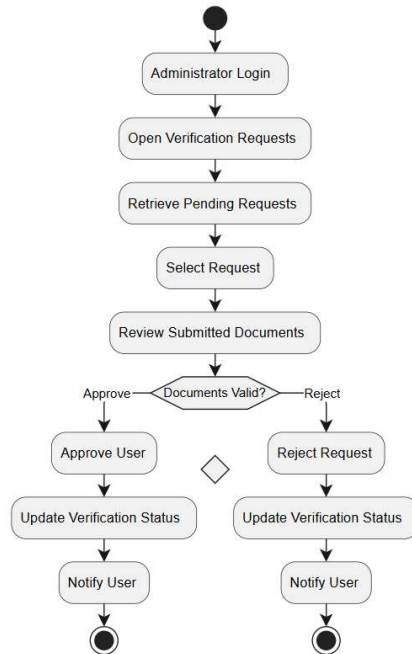
Figure 45- Activity Diagram – Manage Verification Requests
